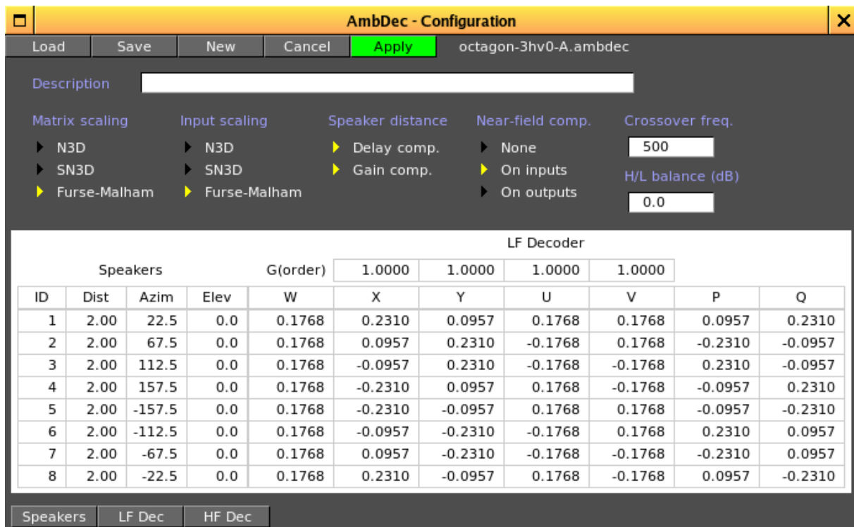
Figure 3: The configuration window, showing decoder matrices
